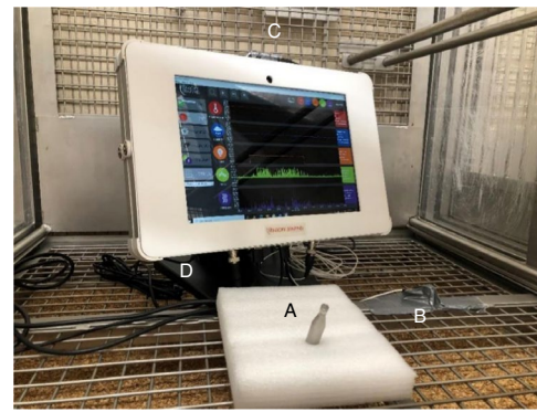
Fig. 1 | Sensory Sentinel device setup shown inside of a modular primate cage unit. Microphone (PCB 426A11 ICP) mounted in an upright, outward-facing direction using styrofoam (A). Accelerometer (PCB 353 C33) taped to floor of cage (B). Light sensor mounted on top of device angled in direction of light source (C). Temperature and humidity sensor (not visible) mounted on the base of the device (D).
