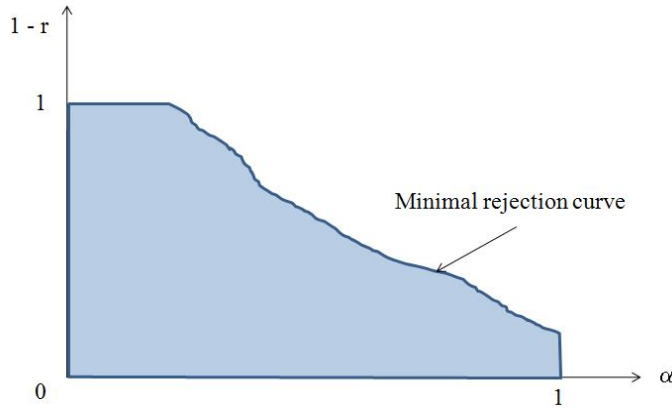
Figure 1: Alternative Equilibrium Rejection Probabilities
