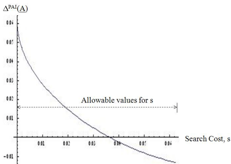
Figure 2: Net Welfare vs. Search Cost
