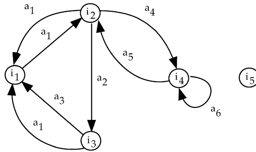
Fig. 1. Network G .
