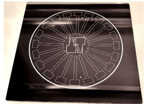
Chrome – glass dark field mask used to fabricate graphene biosensors that probe electrical activity in the brain
