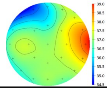
Thickness map demonstrating good uniformity of 37nm \text{Al}_2\text{O}_3 ALD film across 6 inch wafer.
